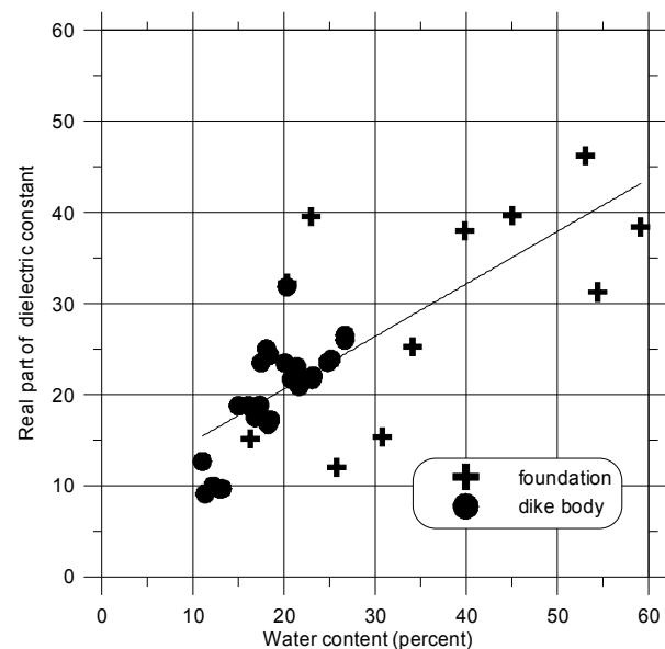
Figure 5. Relation between water content and real part of dielectric constant at 100 MHz.
