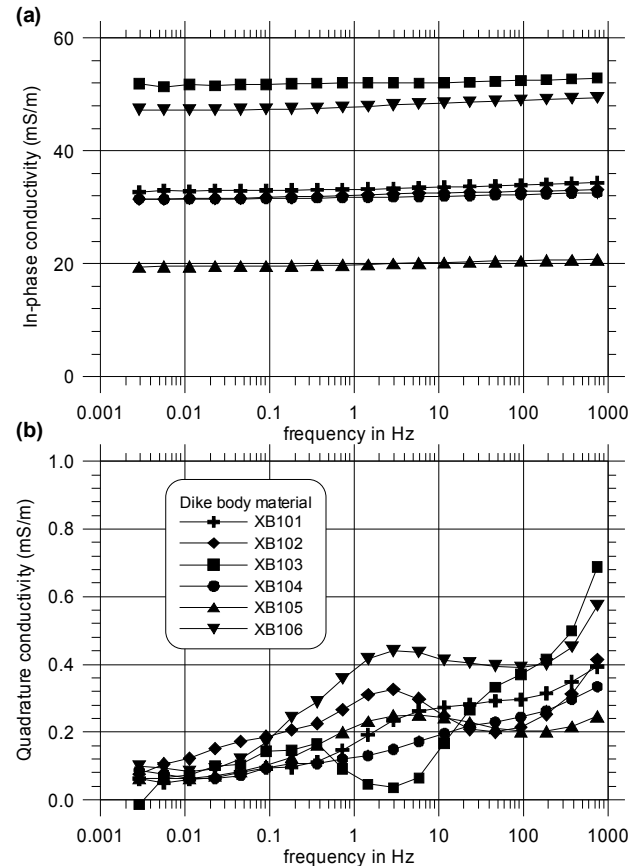
material from dike cross-section at km 138.358. (a) In-phase conductivity. (b) Quadrature conductivity.
