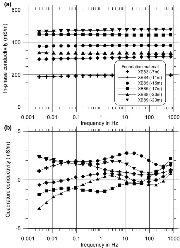
Figure 2. Complex conductivity spectra of material from dike foundation. The samples are taken from the borehole at km 138.358. (a) In- phase conductivity. (b) Quadrature conductivity.
