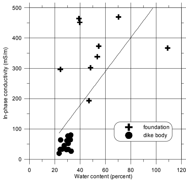
Figure 4. Relation between water content and in-phase conductivity at 2.9 Hz.
