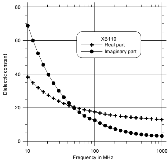
Figure 1. Dielectric spectra of sample XB 110.
